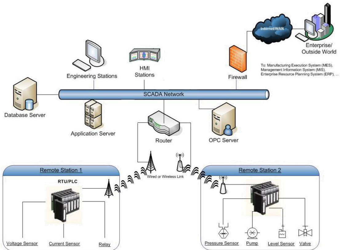
OpenControl SCADA Network Architecture
